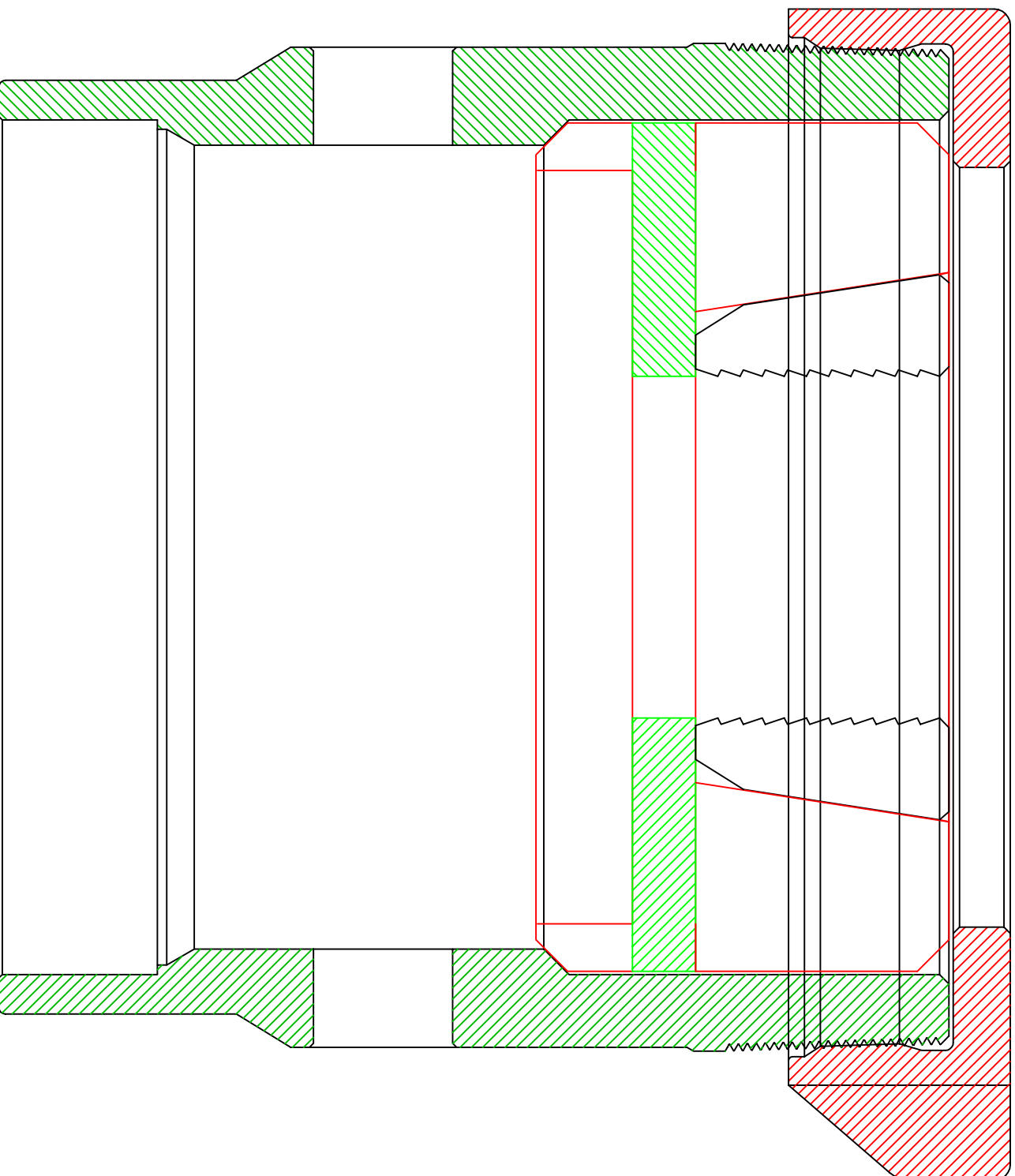
13- \frac{3}{8} SOW Body Carbon Steel P/N 9213-0000-031
