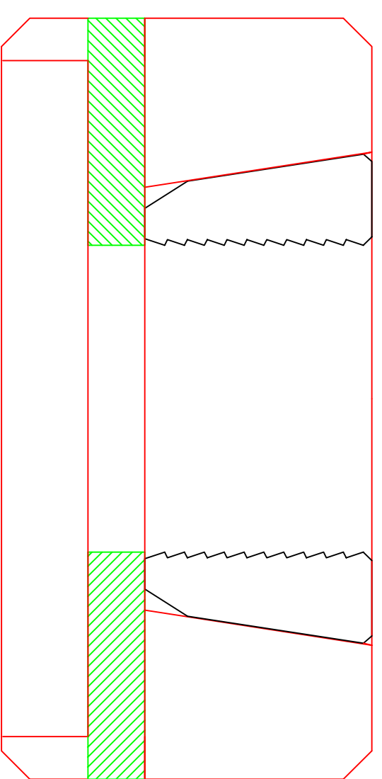
C-22 13- \frac{3}{8} X 5- \frac{1}{2} Hanger, Load Activated Slip Assembly. Max. Load 250,000# P/N 9213-0055-022
