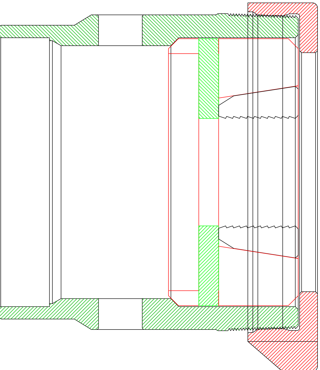
13- \frac{3}{8} SOW Body Carbon Steel P/N 9213-0000-031
