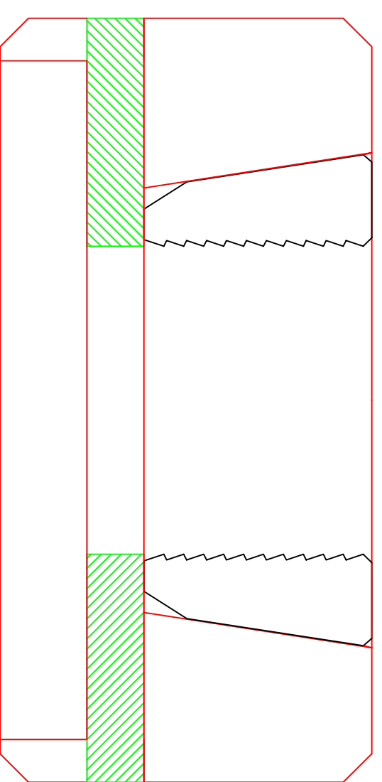
C-22 13- \frac{3}{8} " X 9- \frac{5}{8} " Hanger, Load Activated Slip Assembly. Max. Load 250,000# P/N 9213-0958-022
