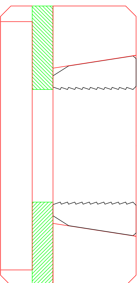
C-22 10- \frac{3}{4} " X 5- \frac{1}{2} " Hanger, Load Activated Slip Assembly. Max. Load 250,000# P/N 9210-0055-022
