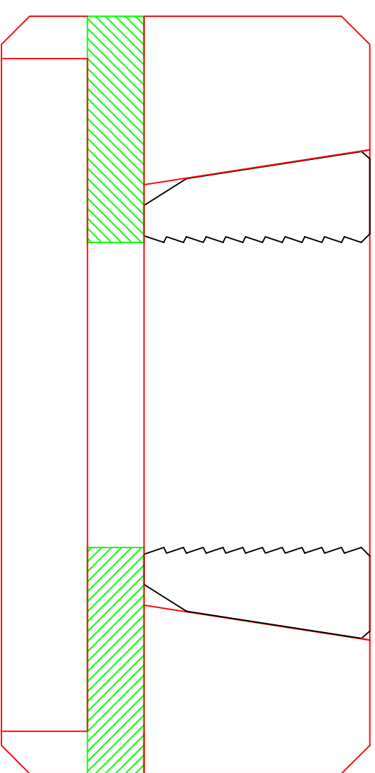
C-22 10- \frac{3}{4} " X 4- \frac{1}{2} " Hanger, Load Activated Slip Assembly. Max. Load 250,000# P/N 9210-0045-022
