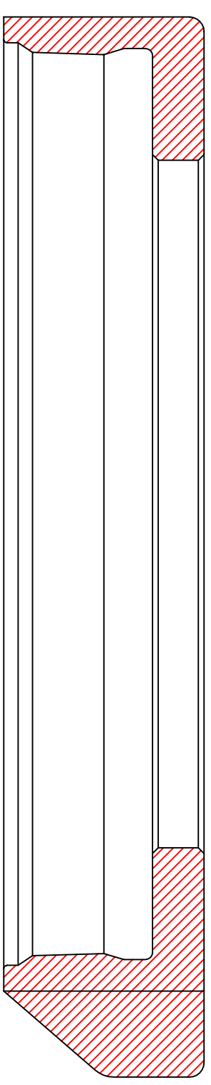
12- \frac{3}{4} " 8V Top Cap P/N 9210-0010-016
