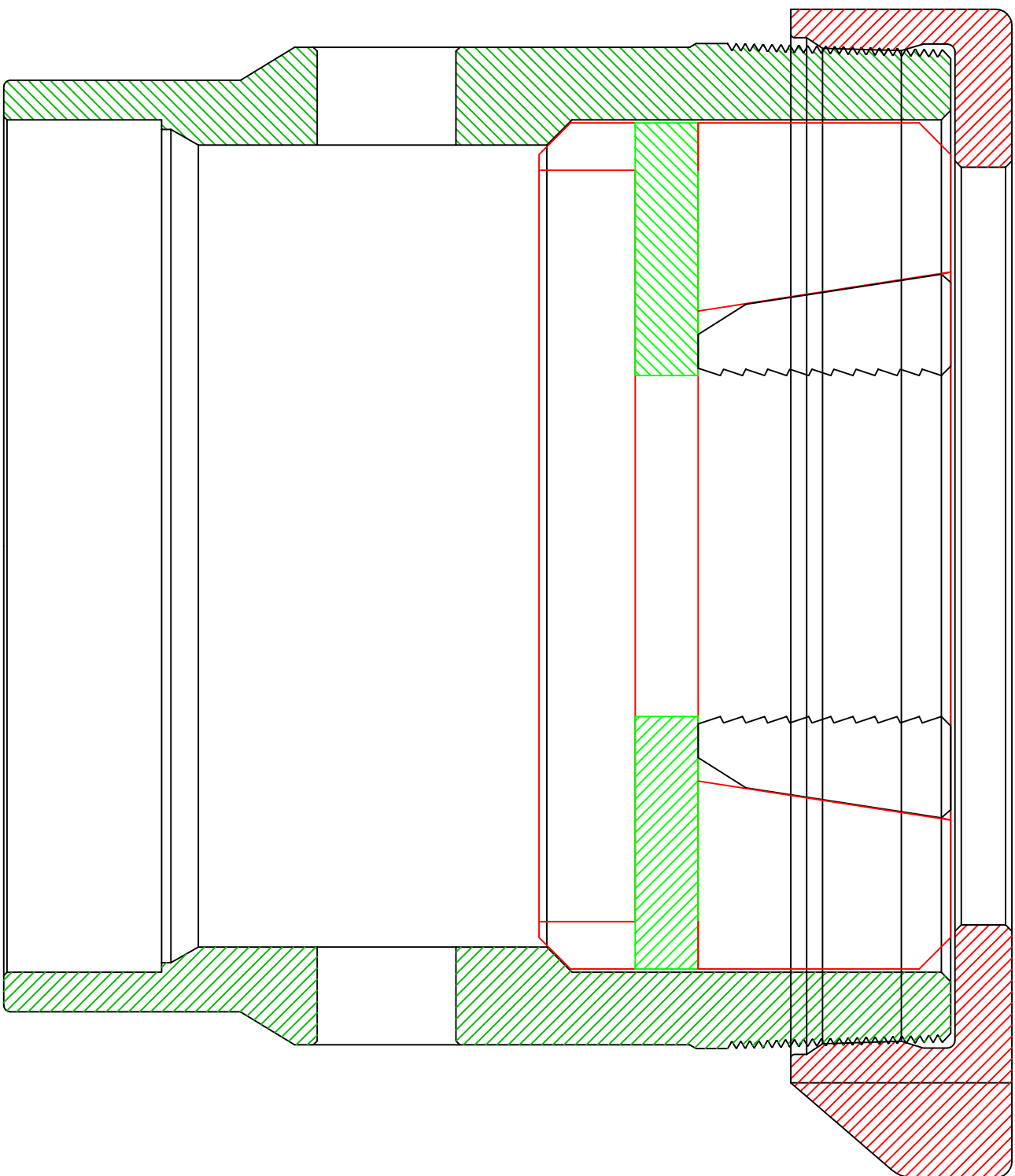
10- \frac{3}{4} " SOW Body Carbon Steel P/N 9210-0000-031
