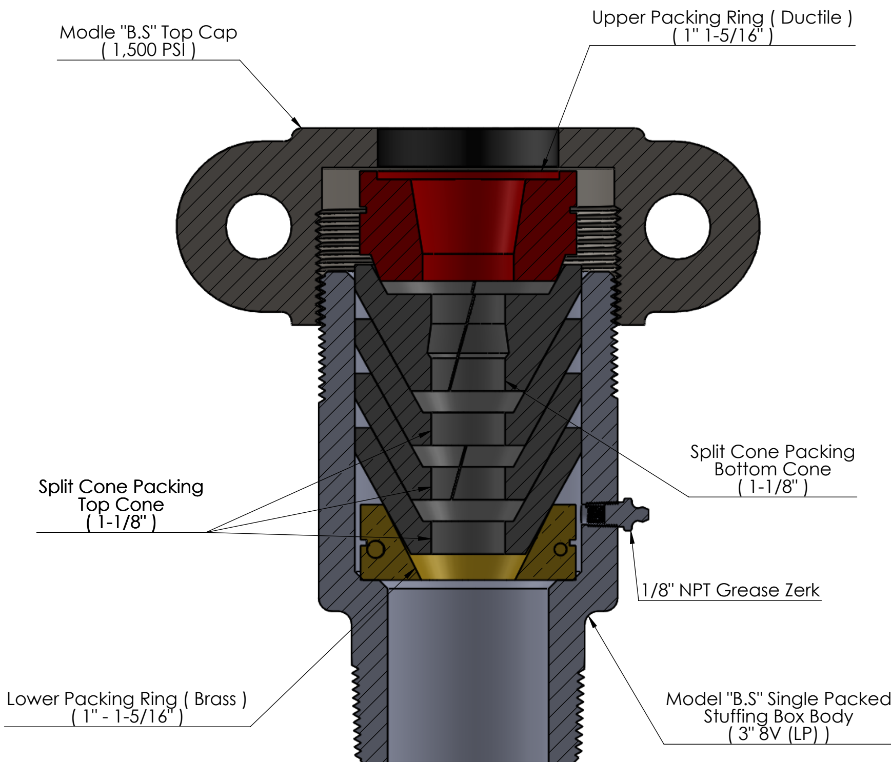
SECTION O-O SCALE 1 : 1.5
