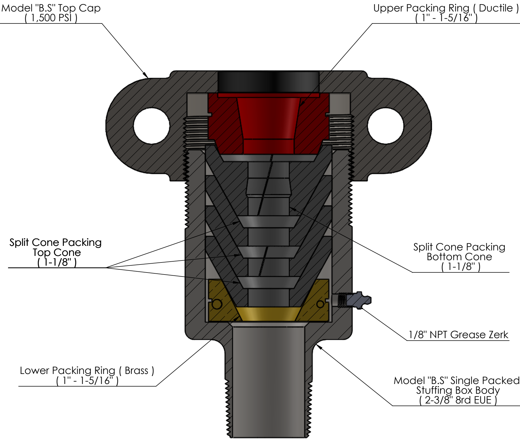
SECTION N-N
