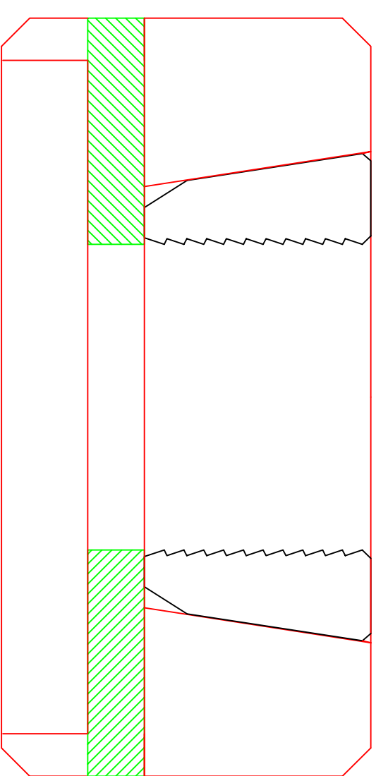
C-22 13- \frac{3}{8} X 7" Hanger, Load Activated Slip Assembly. Max. Load 250,000# P/N 9213-0070-022
