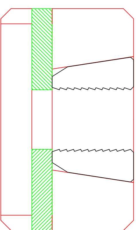
C-22 11" X 7" Hanger, Load Activated Slip Assembly. Max. Load 250,000# P/N 9210-0070-022
