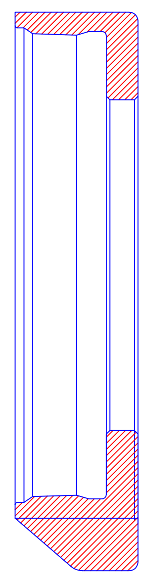
12- 3 / 4 " 8V Top Cap P/N 9210-0010-016
