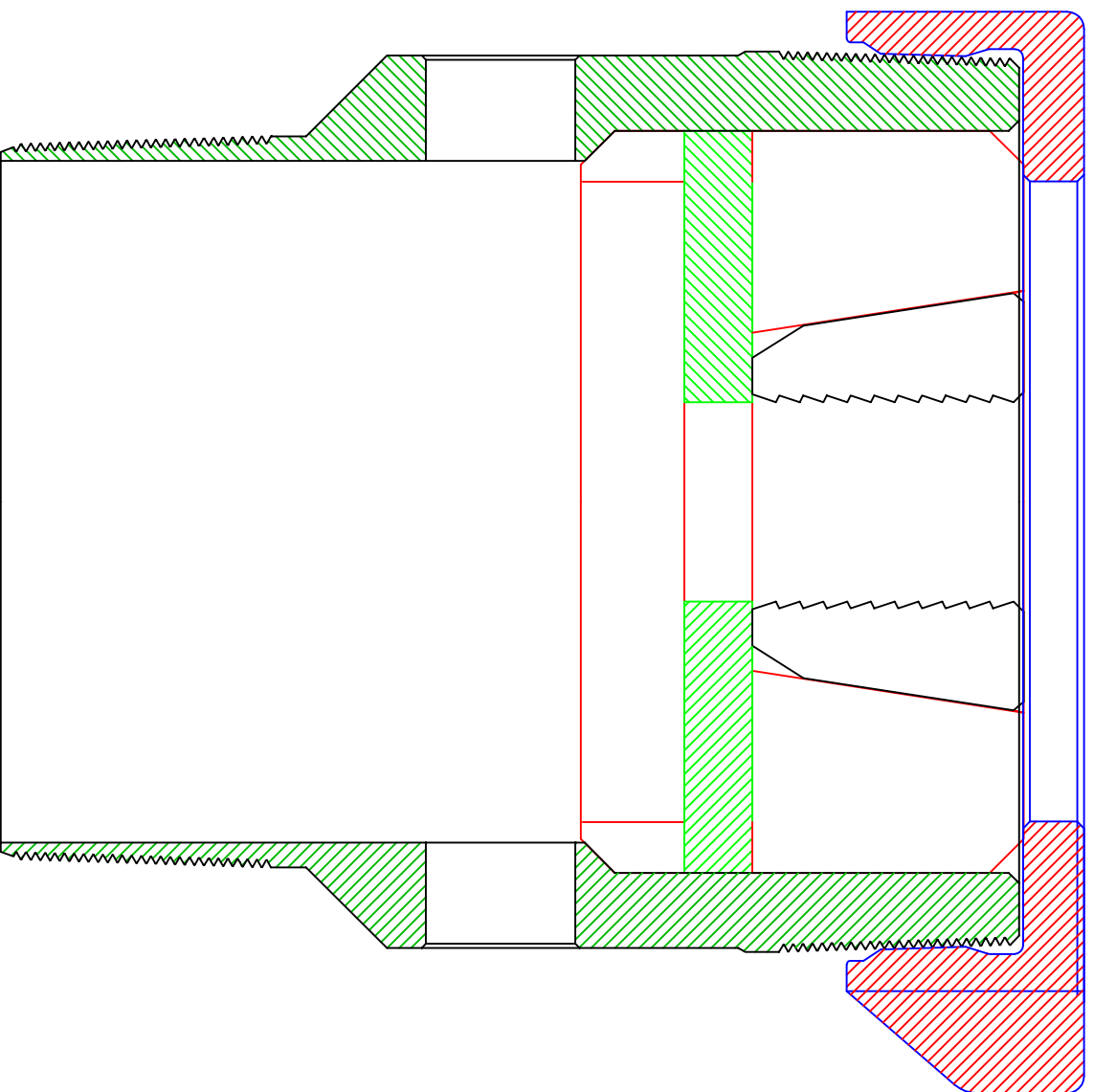
10- 3 / 4 " 8rd Body Carbon Steel P/N 9210-0000-030
